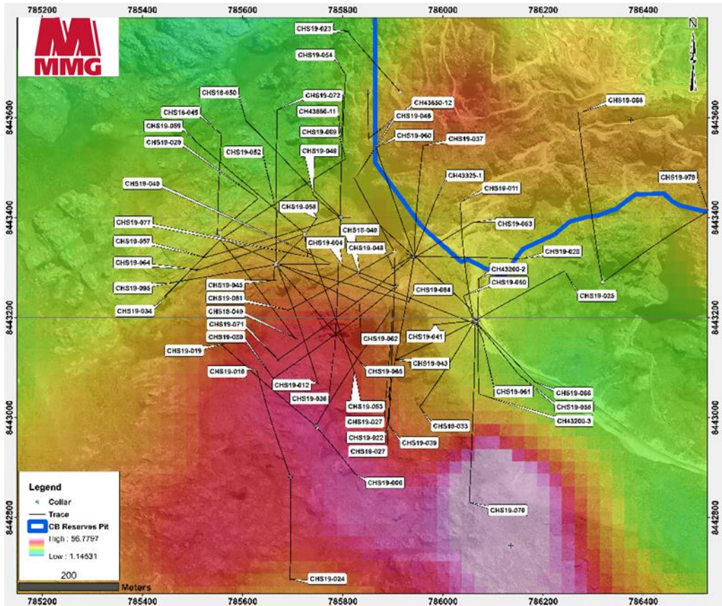
Figure 3. Same area shown in Figures 1 & 2 with base map of IP Chargeability depth slice at 200 meters.
