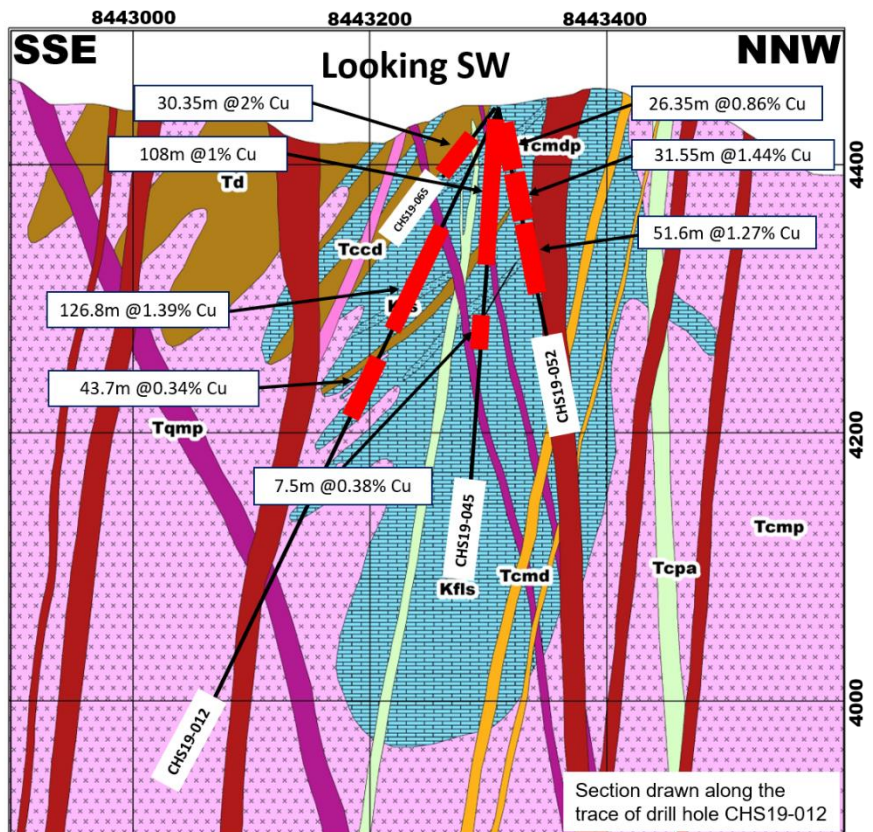
Figure 4. Geologic Cross Section through drill hole CHS19-012. Refer to Figure 2 for drillhole location.
