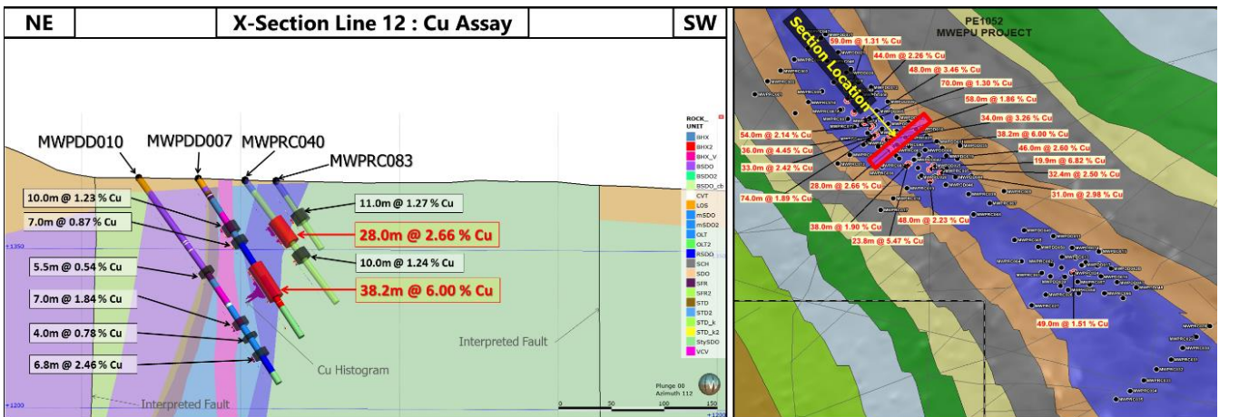
Figure 11: Mwepu Project: Representative cross section – Line 12.
