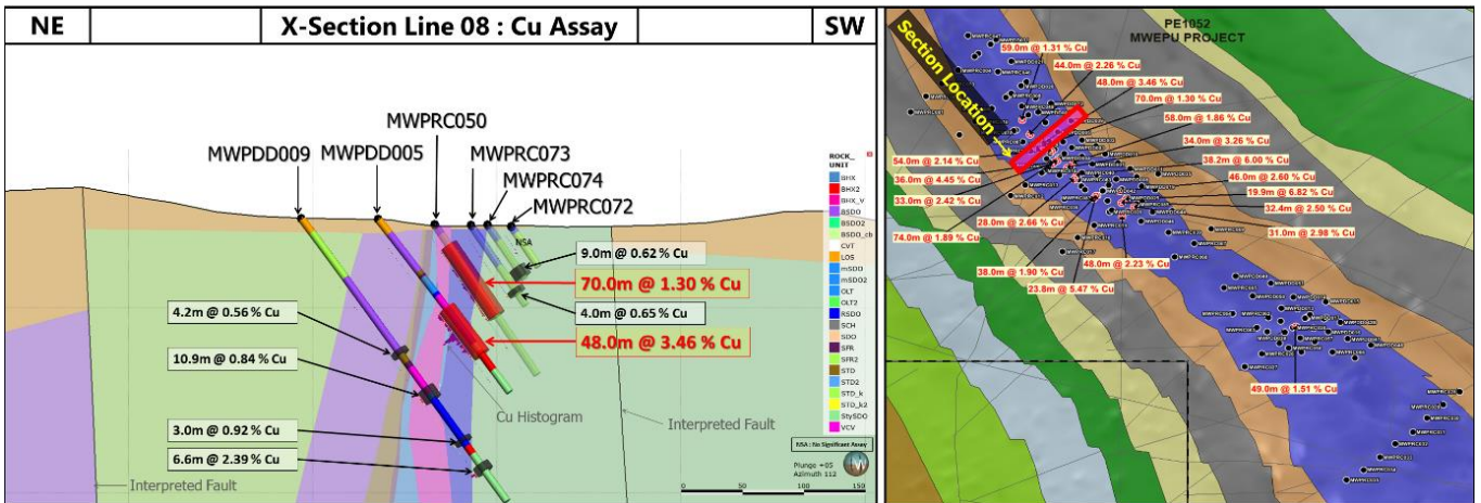
Figure 9: Mwepu Project: Representative cross section – Line 08.
