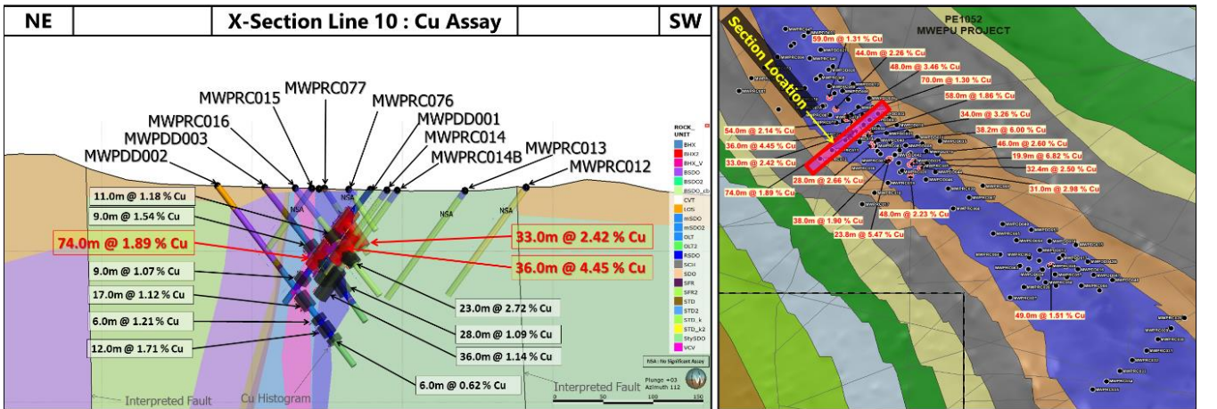
Figure 10: Mwepu Project: Representative cross section – Line 10.
